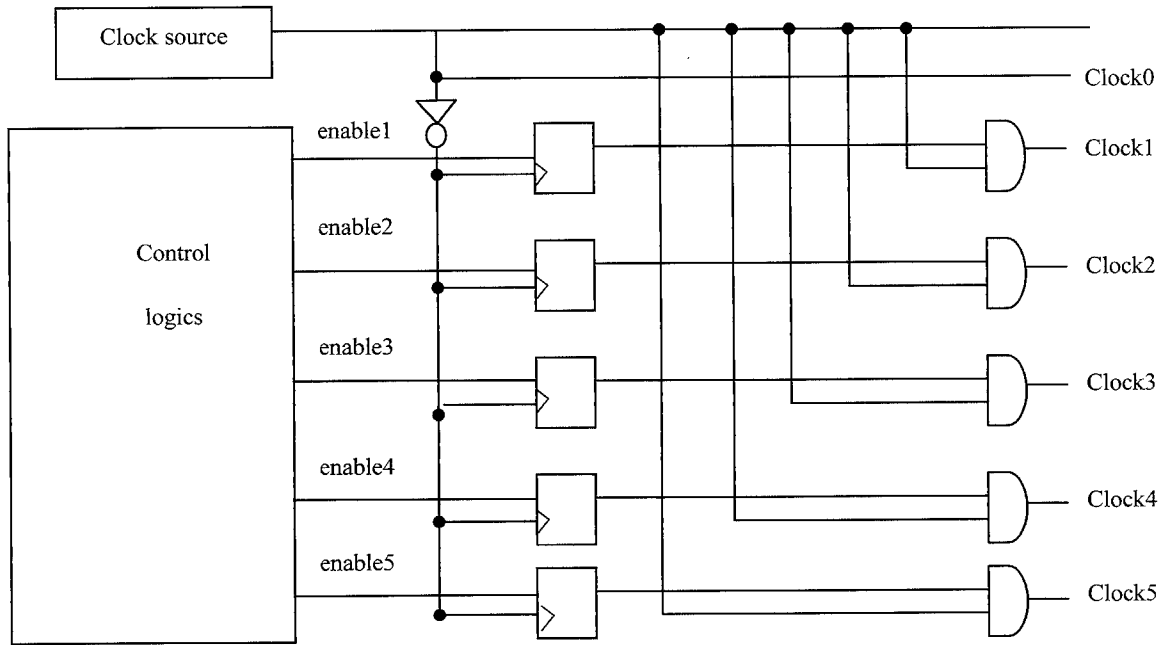
Fig.3 The architecture of the clock enabling circuit of a wireless communication chip which is used as an example in this paper. All 6 clocks are originated from the same clock source.
