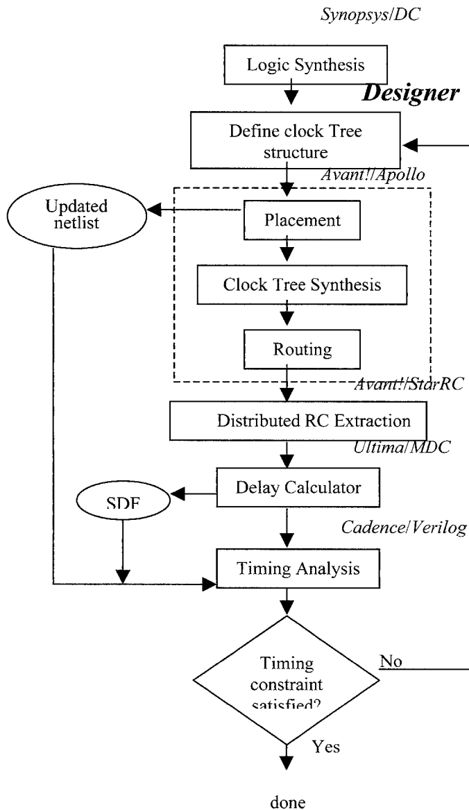
Fig.2 Clock Tree Synthesis Design
