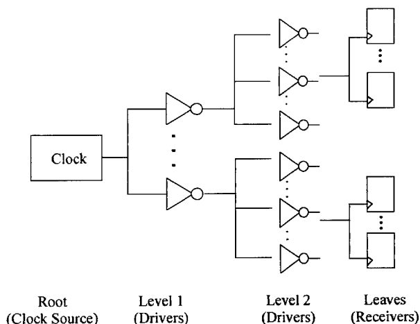
Fig.1 A two level clock Tree structure
