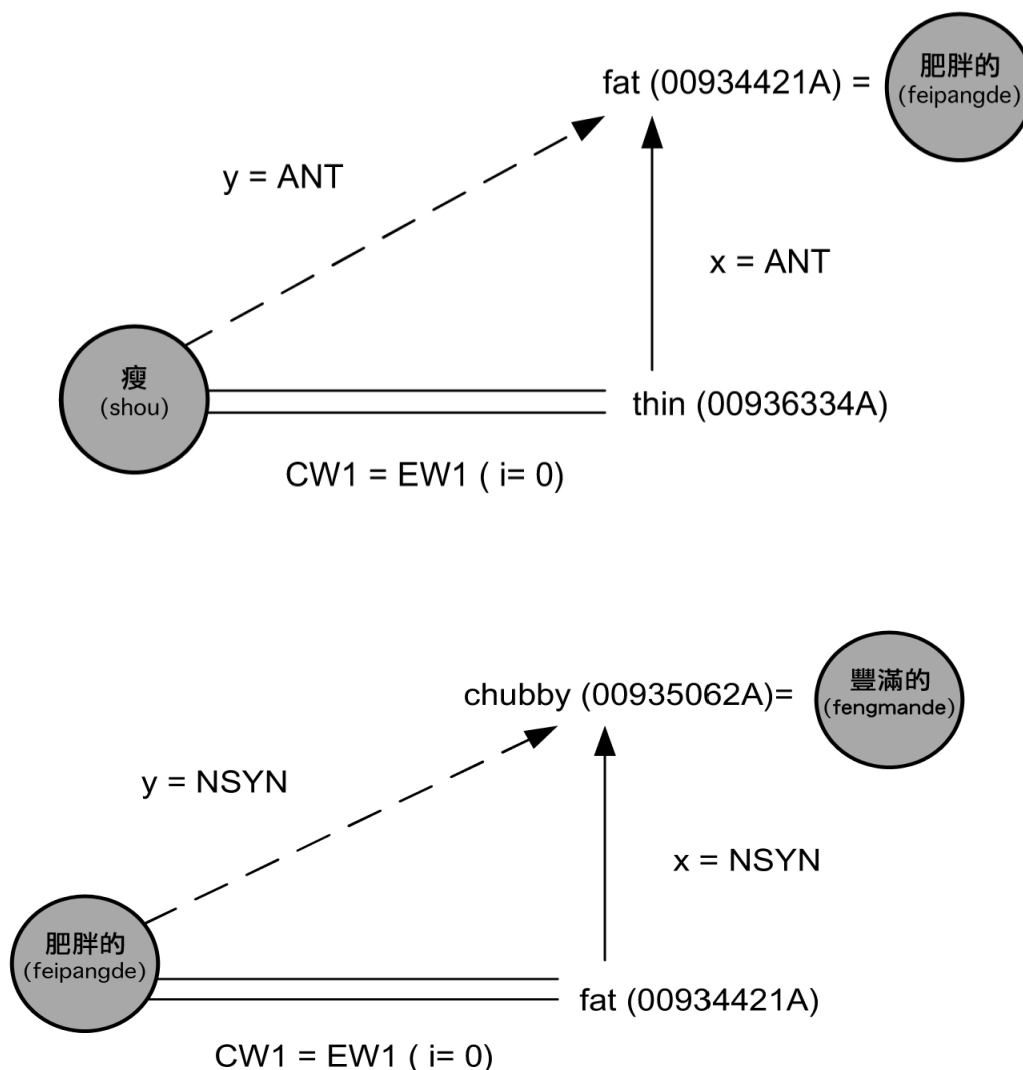
Figure 3. Translation-mediated LSR (when TEs are synonymous): The unknown LSR\ y = \theta + x = x
